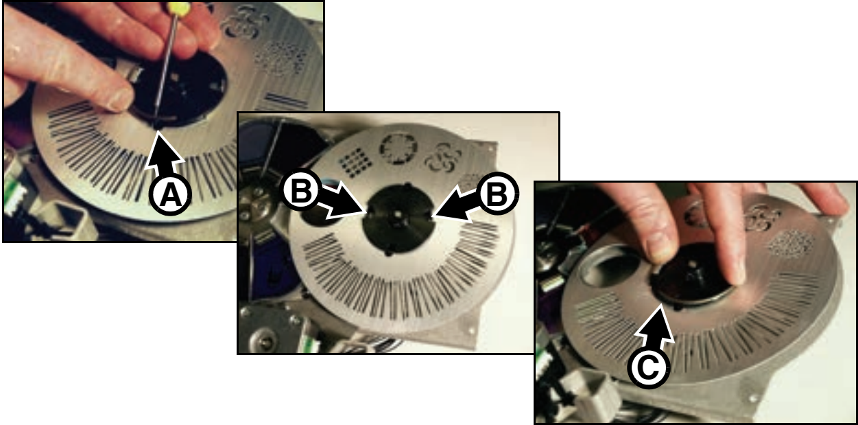
Figure 27: FX wheel removal and mounting
