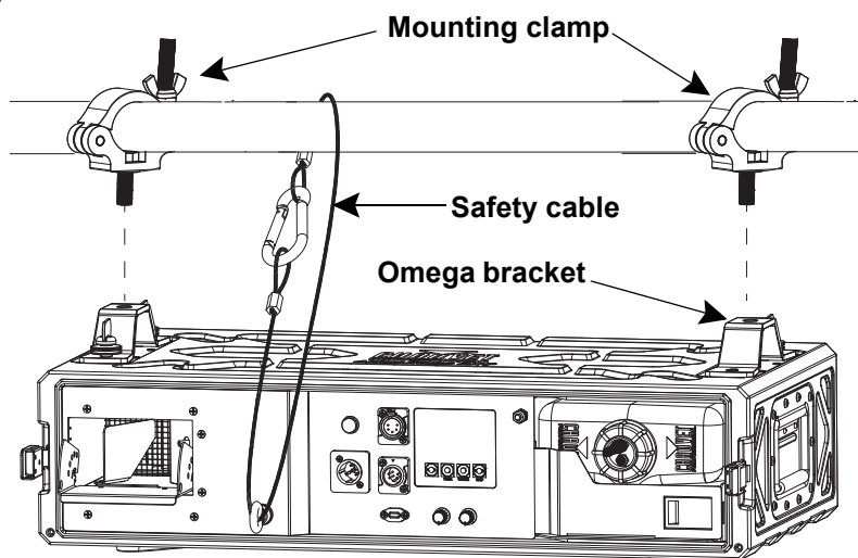
Overhead Mounting
